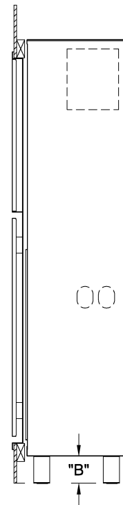
Side Cutaway View
