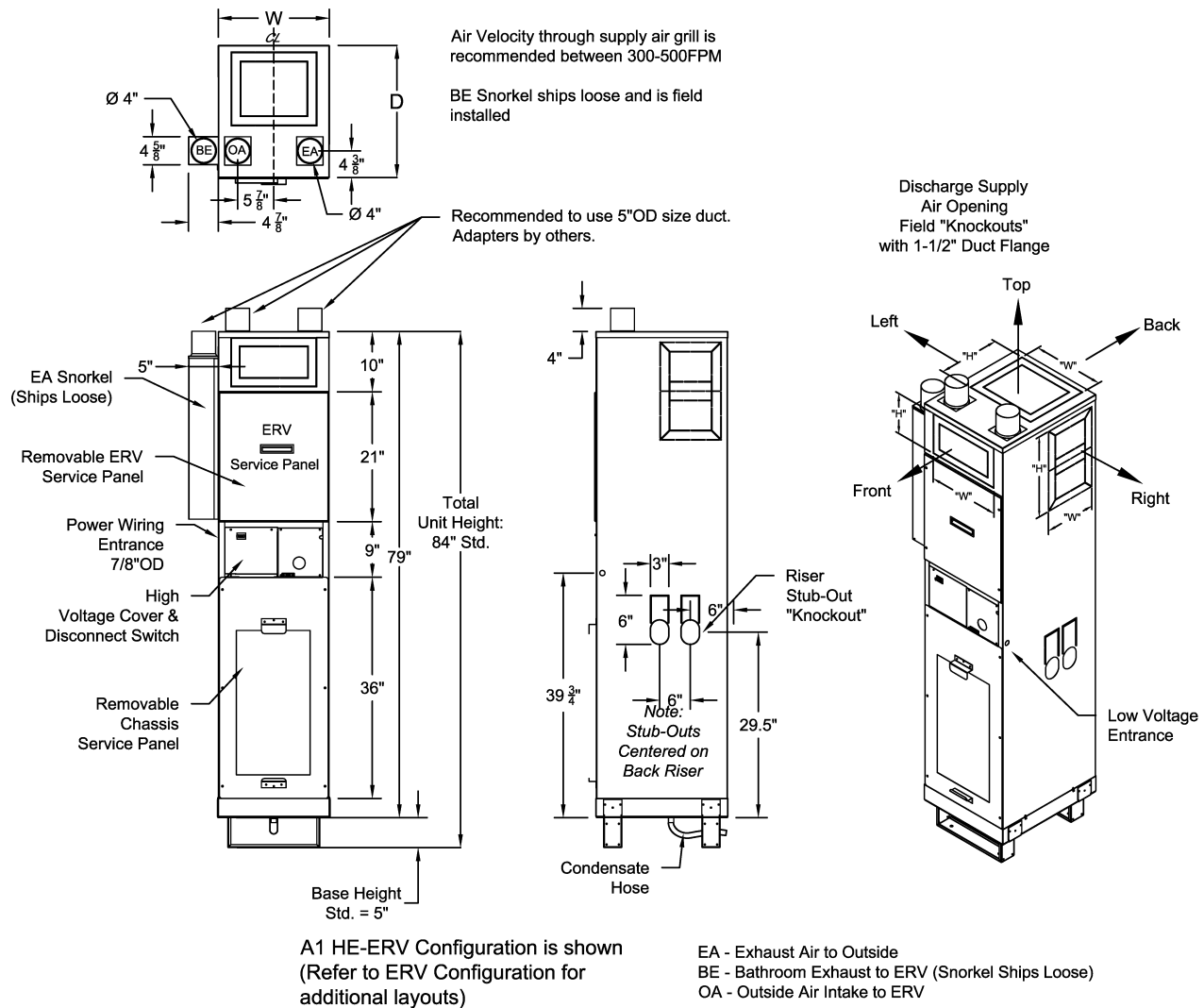
VSHYe Cabinet Dimensions
